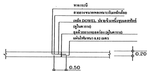
EXPANSION JOINT
