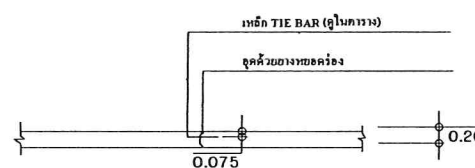
LONGTUDINAL JOINT
